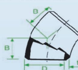
45° LR Elbows
