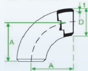
90° LR Elbows
